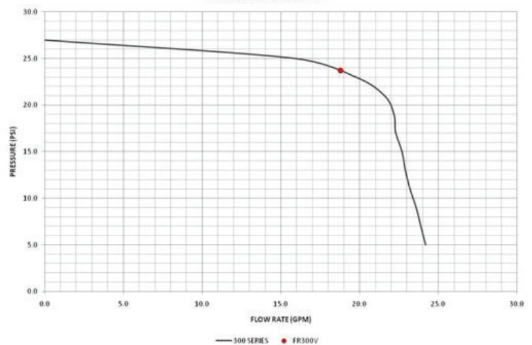
300 SERIES PERFORMANCE CURVE
